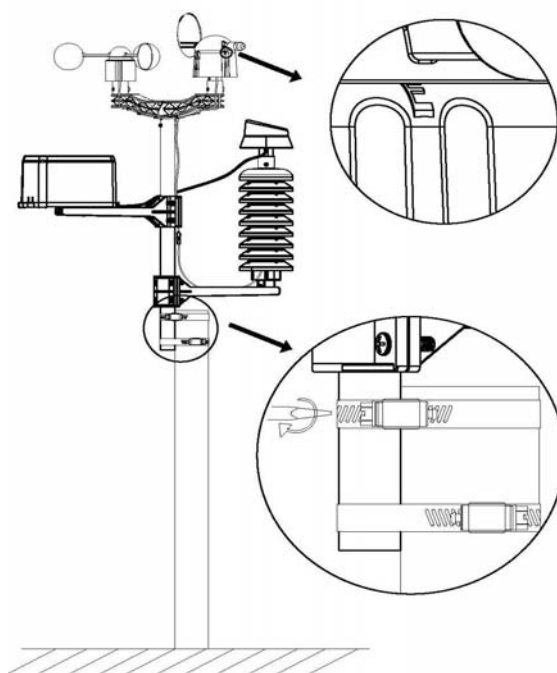
Fix the whole set to a pole with the two adjustable hoops.
